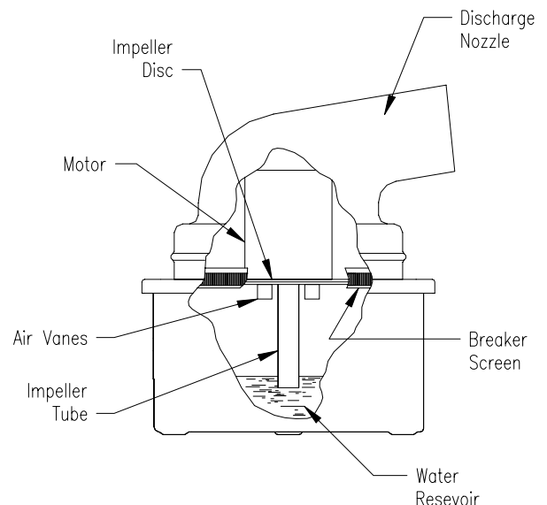
Centrifugal Atomizer
